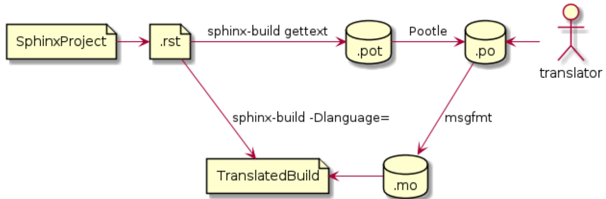
Fig. 1: Workflow visualization of translations in Sphinx. (The figure is created by plantuml Page 188, 290. )
